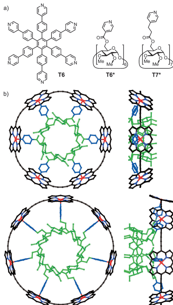
Figure 1. a) Rigid T6 and flexible T6* and T7* cyclodextrin templates. b) Geometries of c-P6-T6* and c-P7-T7* from small-angle X-ray scattering and molecular mechanics calculations (MM + force field, orthogonal views, meso -aryl groups and hydrogen atoms are omitted for clarity).
